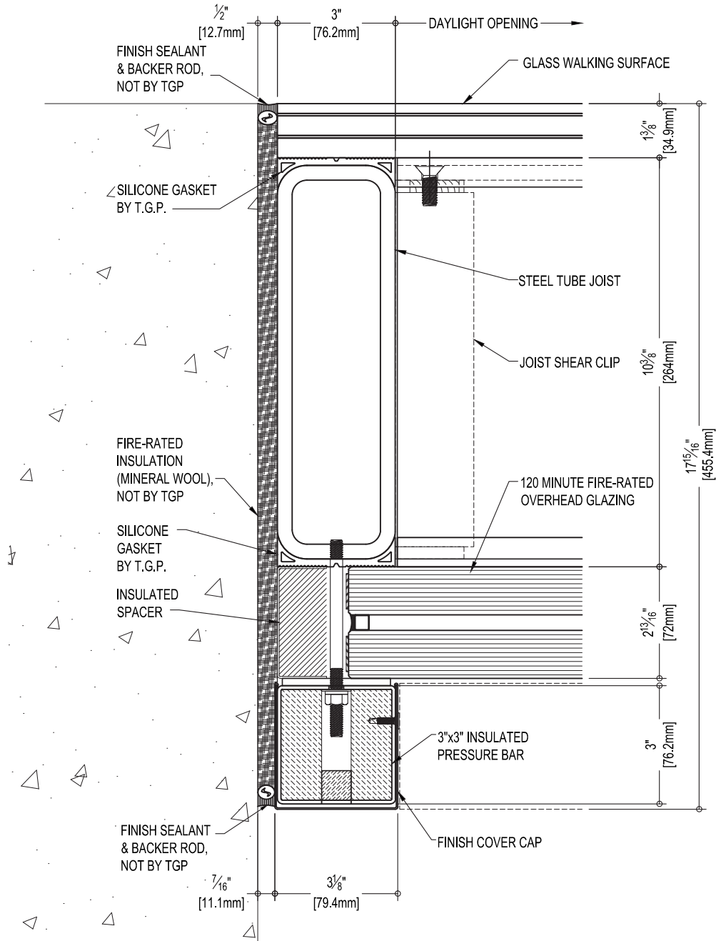
1 LONG JOIST CROSS SECTION AT EDGE CONDITION
