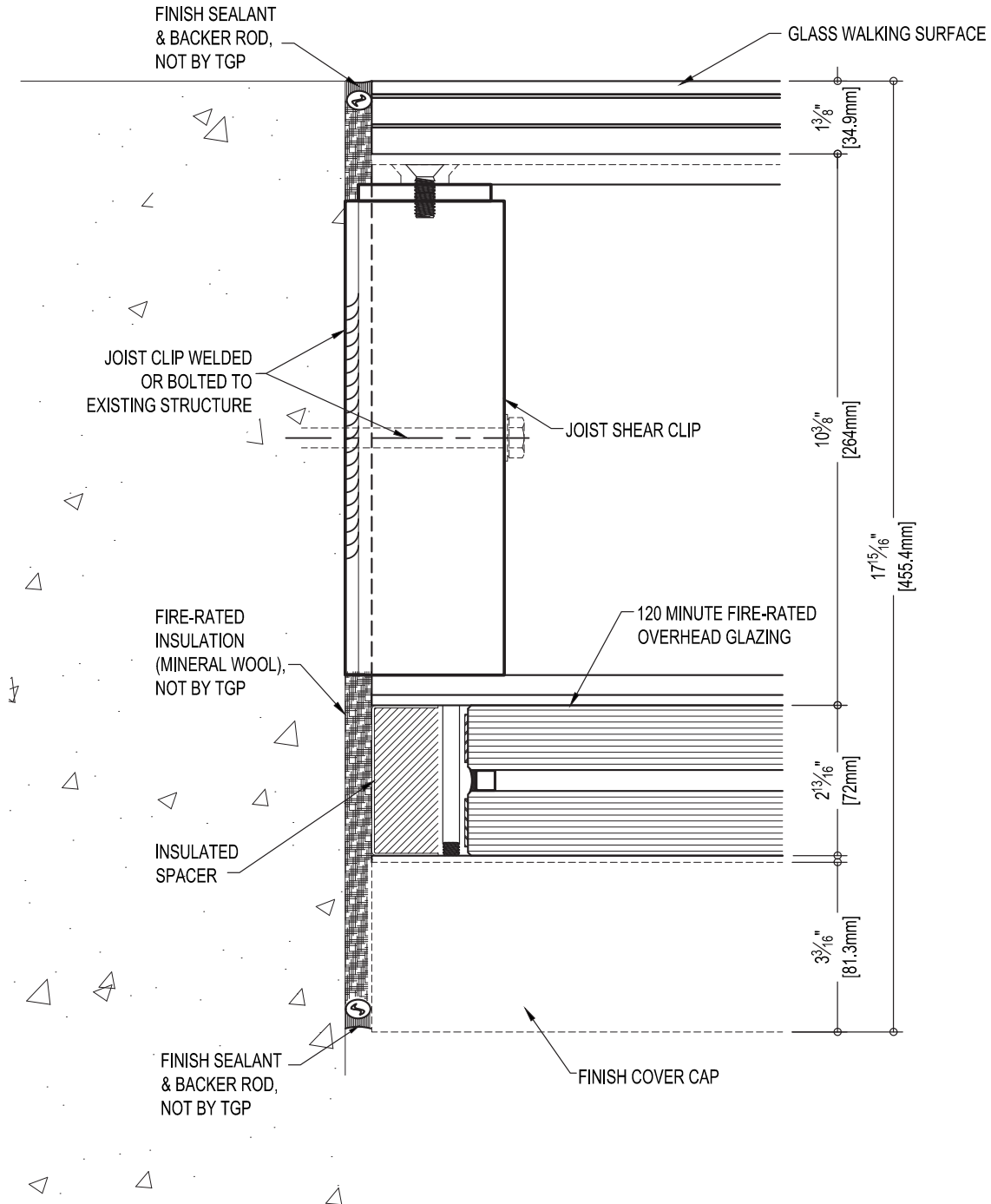
3 JOIST CROSS SECTION AT JOIST ANCHOR
